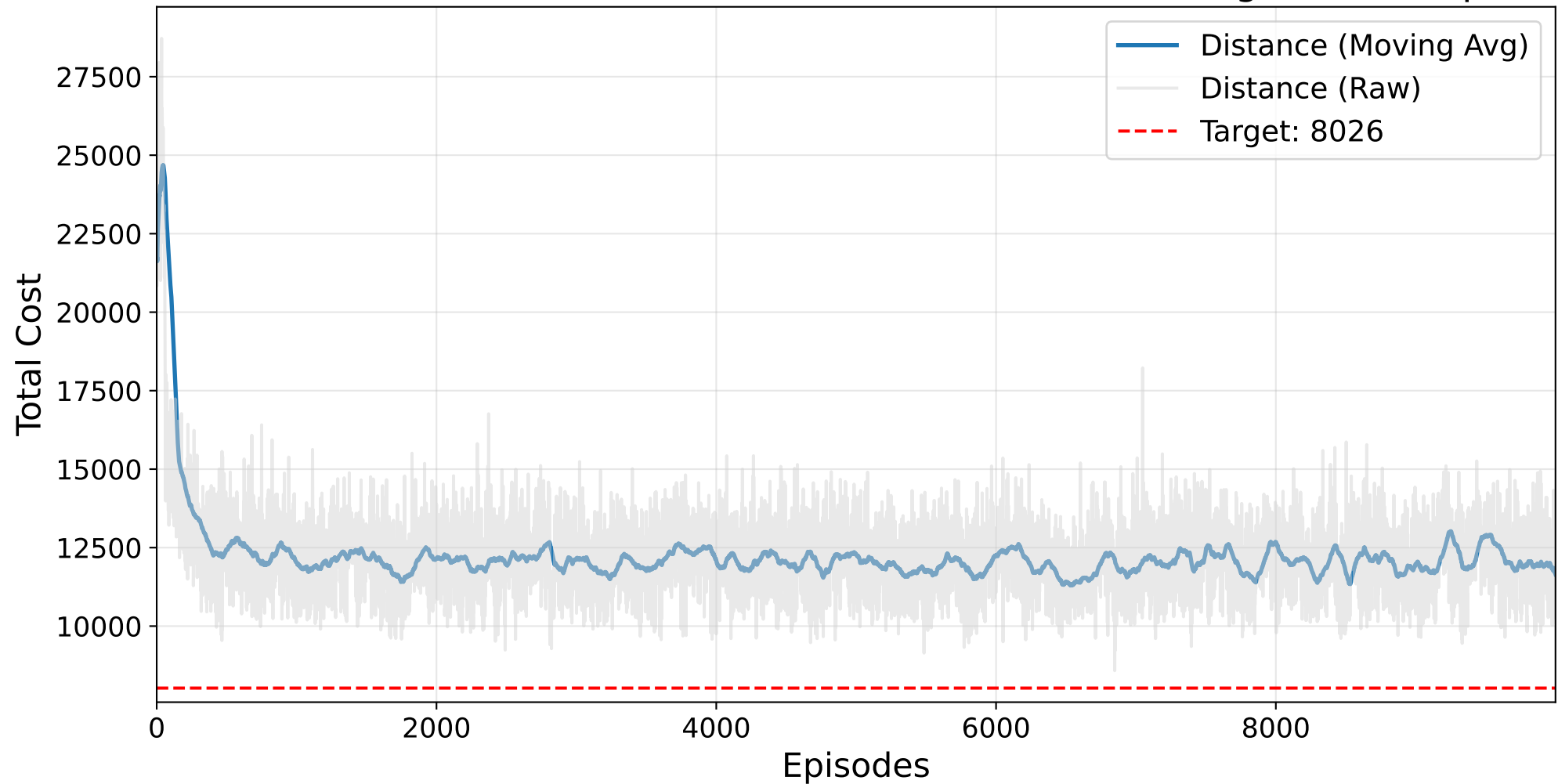
Final GAUSSIAN PROCESS Masked AutoRL-SOP Training - ft53.2.sop
